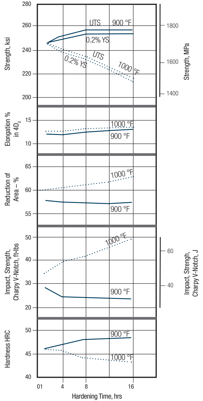
FIGURE 40 – COLD REDUCED 20%
