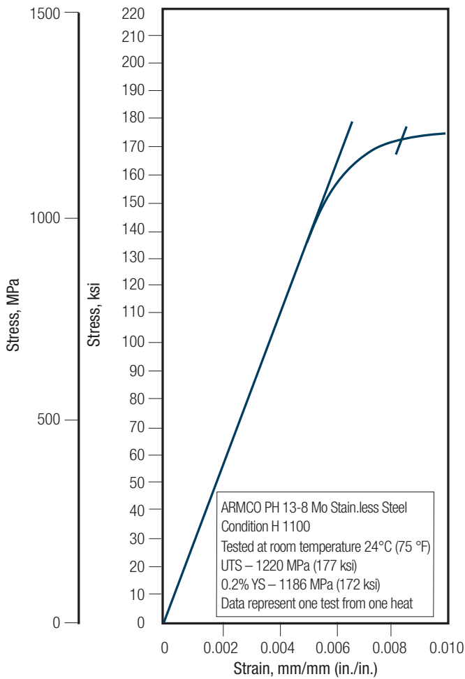
FIGURE 25 – EFFECT OF VARIOUS HEAT-TREATED CONDITIONS ON ROOM TEMPERATURE CURVES – TENSION
