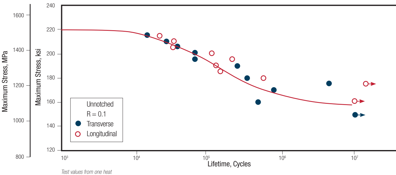
FIGURE 4 – FATIGUE TESTS RESULTS FOR UNNOTCHED LONGITUDINAL AND TRANSVERSE SPECIMENS OF CONDITION H 1000 ARMCO PH 13-8 Mo STAINLESS STEEL AT A STRESS RATIO OF R = 0.1
