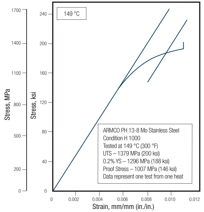
FIGURE 16 – EFFECT OF TEST TEMPERATURE ON CONDITION H 1000 – TENSION
