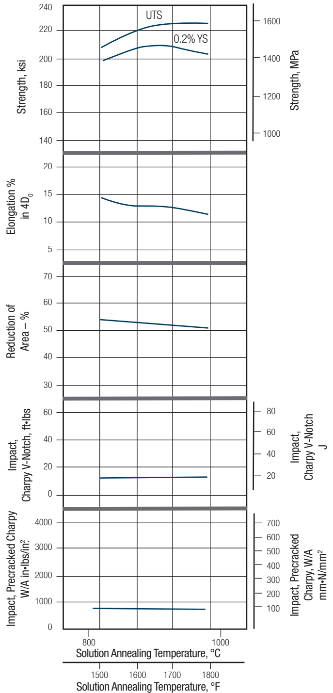
FIGURE 33 – EFFECT OF VARIATION IN SOLUTION TREATMENT* CONDITION H 950
