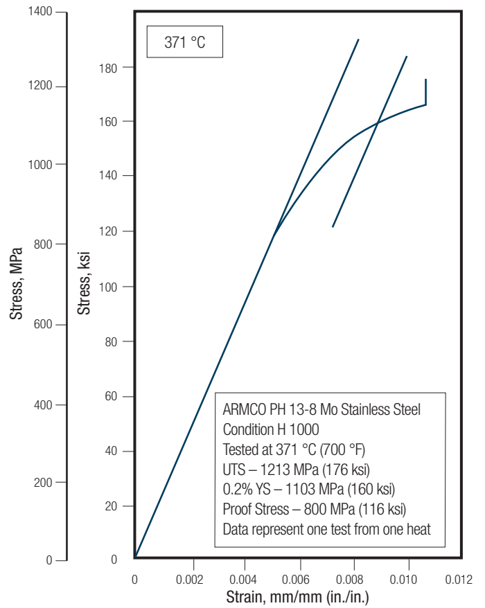
FIGURE 18 – EFFECT OF TEST TEMPERATURE ON CONDITION H 1000 – TENSION
