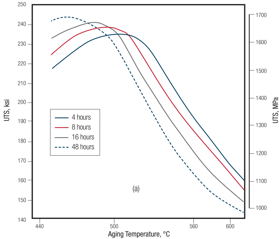
FIGURE 35 – TENSILE STRENGTH VS. HARDENING TEMPERATURE
