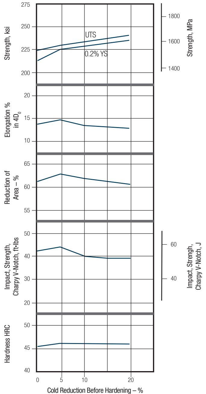
FIGURE 38 – 538 °C (1000 °F) HARDENING TEMPERATURE
