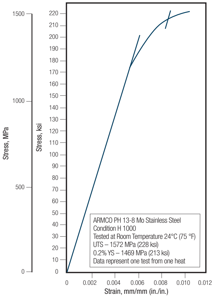
FIGURE 23 – EFFECT OF VARIOUS HEAT-TREATED CONDITIONS ON ROOM TEMPERATURE CURVES – TENSION
