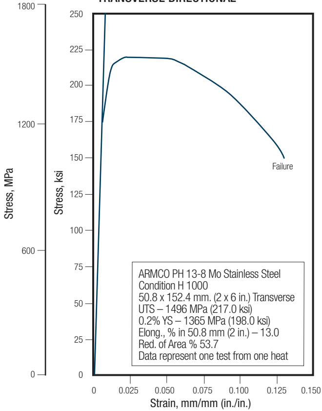
FIGURE 32 – TOTAL STRESS-STRAIN CURVES H1000 TRANSVERSE DIRECTIONAL
