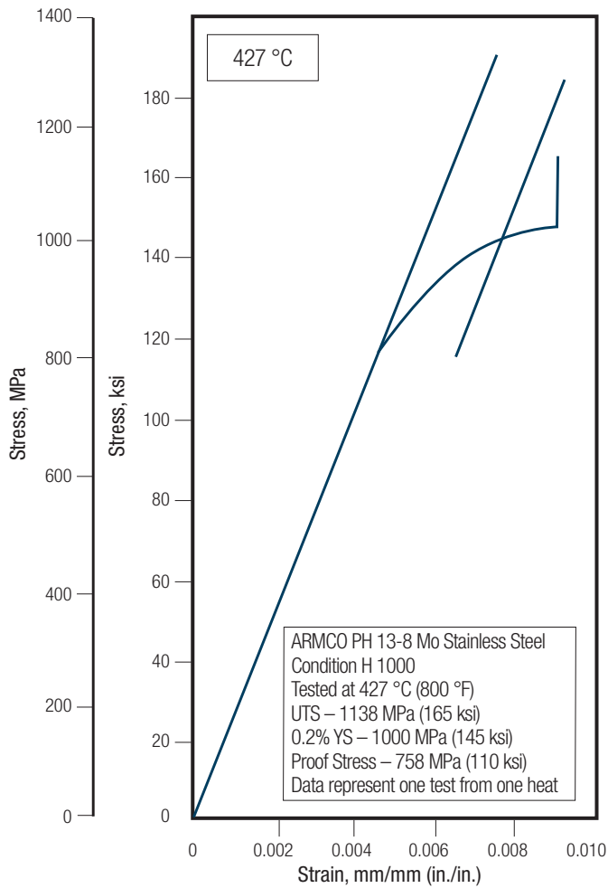
FIGURE 19 – EFFECT OF TEST TEMPERATURE ON CONDITION H 1000 – TENSION
