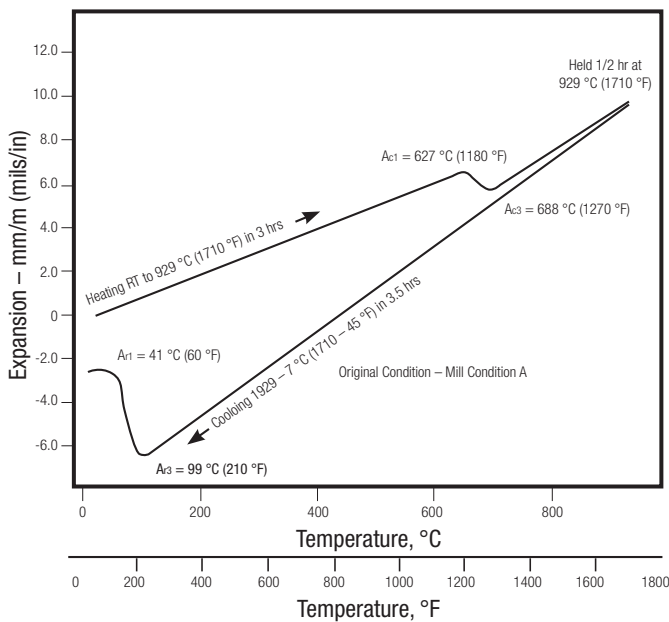
FIGURE 41 – DILATOMETER CURVE
