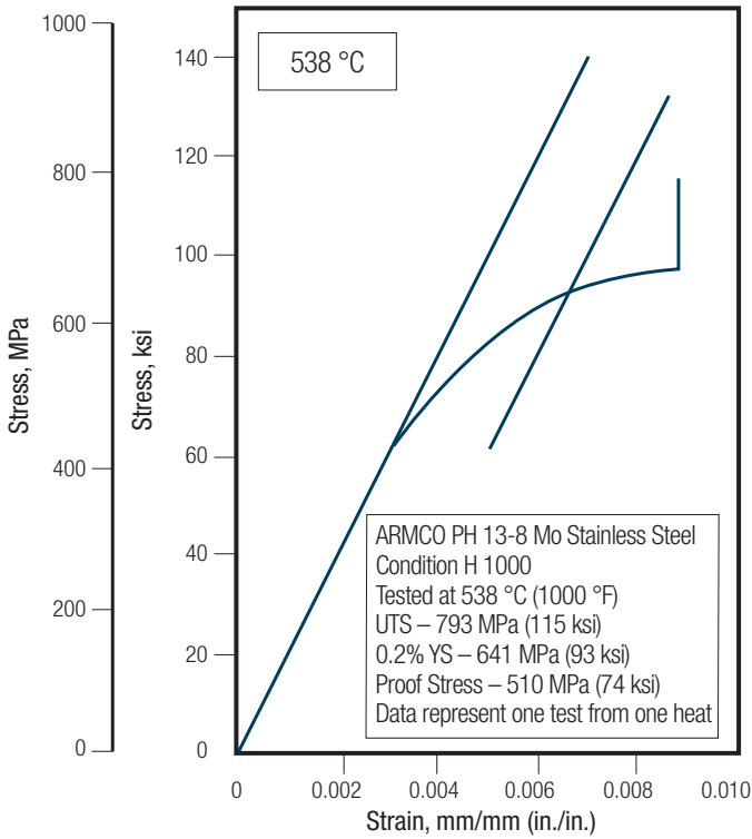
FIGURE 21 – EFFECT OF TEST TEMPERATURE ON CONDITION H 1000 – TENSION
