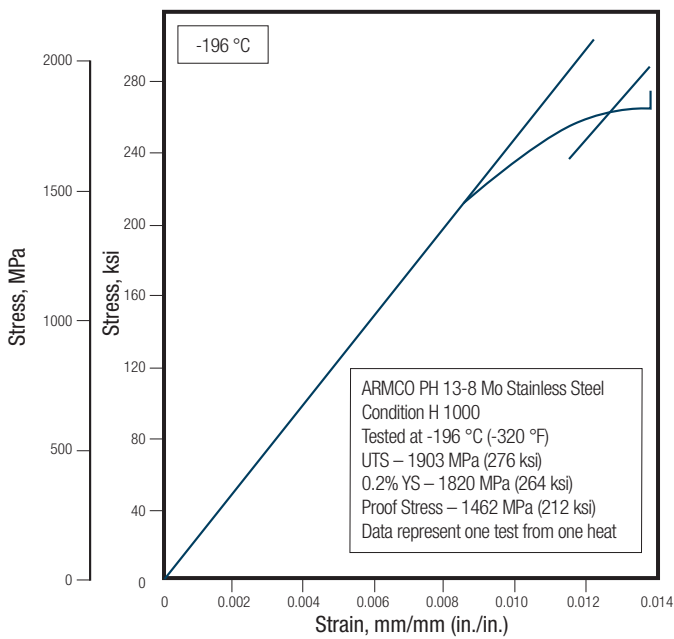
FIGURE 11 – EFFECT OF TEST TEMPERATURE ON CONDITION H 1000 – TENSION
