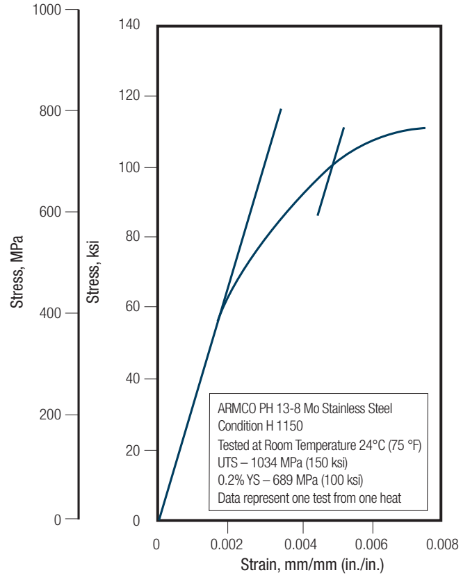
FIGURE 26 – EFFECT OF VARIOUS HEAT-TREATED CONDITIONS ON ROOM TEMPERATURE CURVES – TENSION
