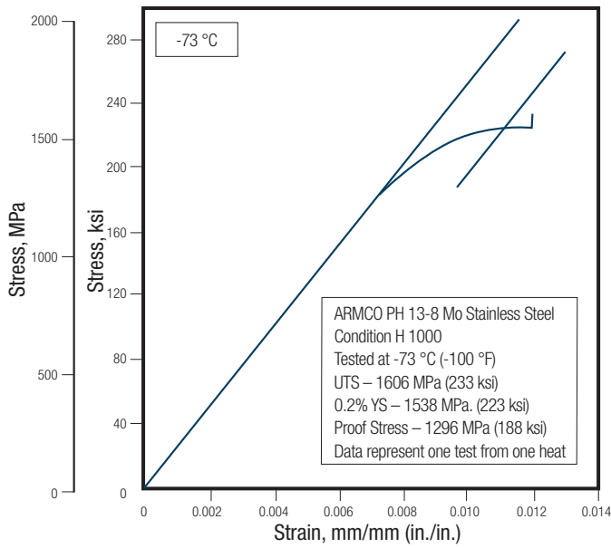
FIGURE 13 – EFFECT OF TEST TEMPERATURE ON CONDITION H 1000 – TENSION
