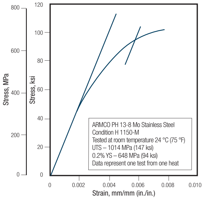
FIGURE 27 – EFFECT OF VARIOUS HEAT-TREATED CONDITIONS ON ROOM TEMPERATURE CURVES – TENSION
