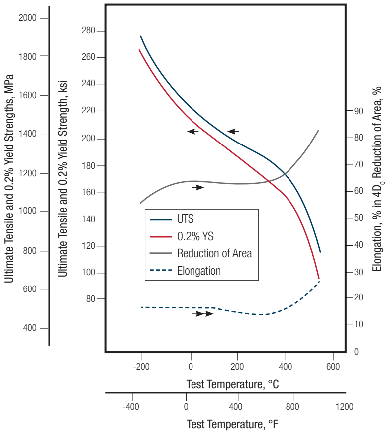
FIGURE 2 – SHORT-TIME ELEVATED TEMPERATURE TENSILE PROPERTIES CONDITION H 1000*
