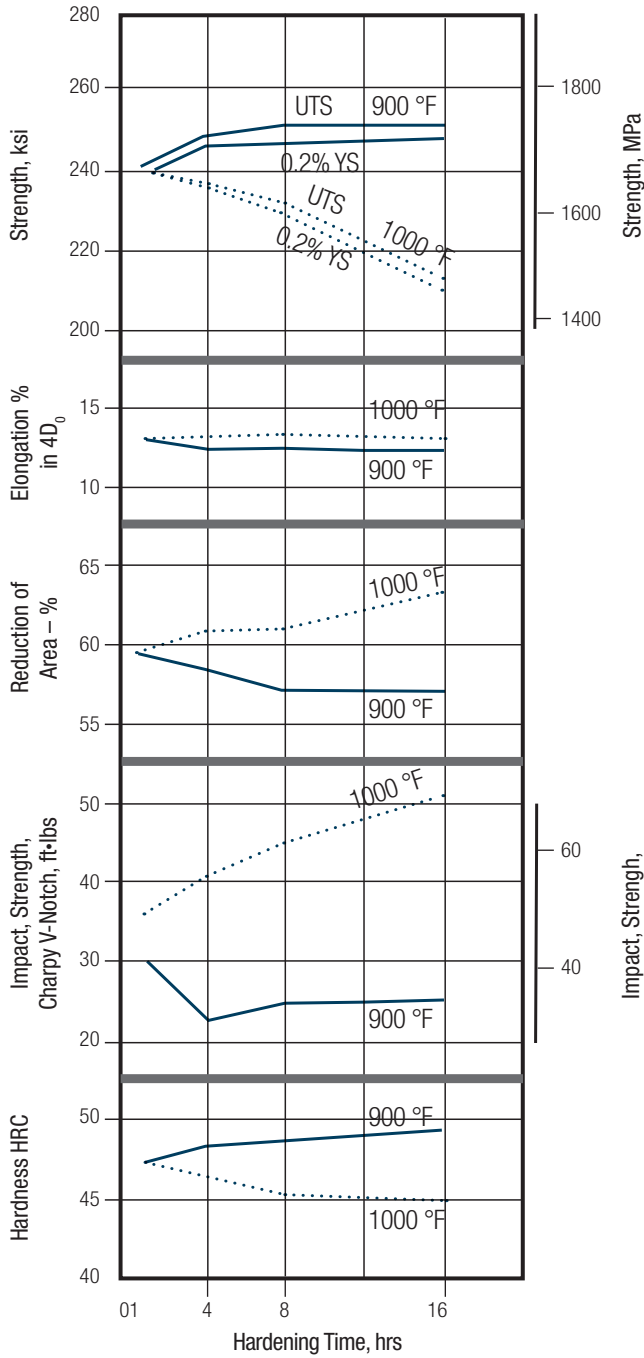
FIGURE 39 – COLD REDUCED 10%
