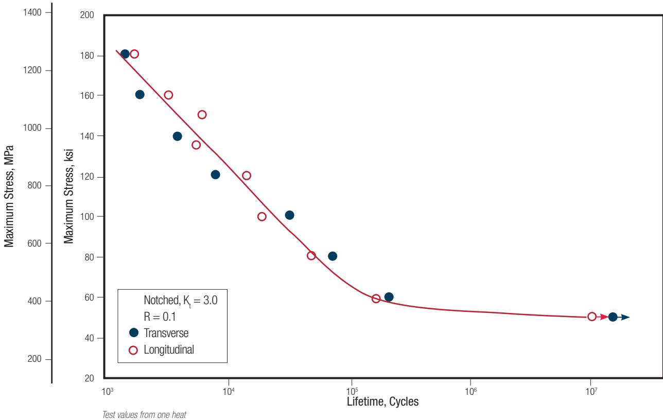
FIGURE 7 – FATIGUE TEST RESULTS FOR NOTCHED ( K_t = 3.0 ) LONGITUDINAL AND TRANSVERSE SPECIMENS OF CONDITION H 1000 ARMCO PH 13-8 Mo STAINLESS STEEL AT A STRESS RATIO OF R = 0.1
