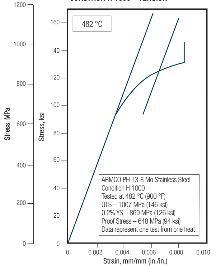
FIGURE 20 – EFFECT OF TEST TEMPERATURE ON CONDITION H 1000 – TENSION
