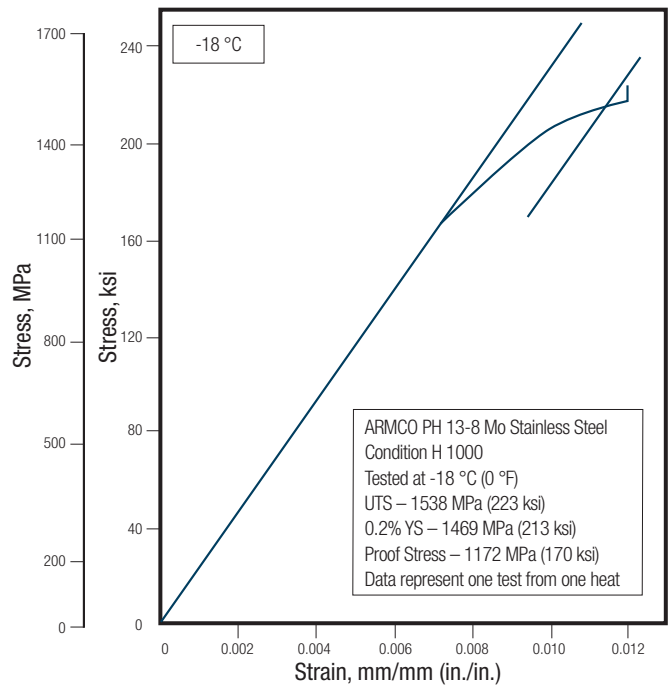
FIGURE 14 – EFFECT OF TEST TEMPERATURE ON CONDITION H 1000 – TENSION
