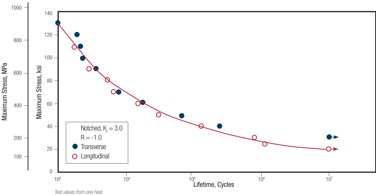
FIGURE 8 – FATIGUE TEST RESULTS FOR NOTCHED ( K_t = 3.0 ) LONGITUDINAL AND TRANSVERSE SPECIMENS OF CONDITION H 1000 ARMCO PH 13-8 Mo STAINLESS STEEL AT A STRESS RATIO OF R = -1.0
