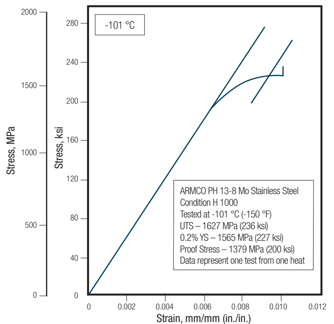
FIGURE 12 – EFFECT OF TEST TEMPERATURE ON CONDITION H 1000 – TENSION
