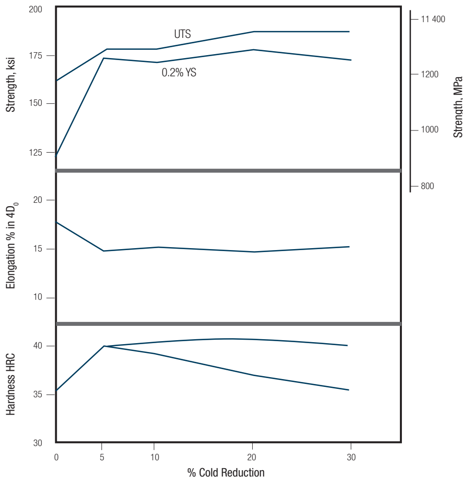
FIGURE 36 – EFFECT OF COLD WORK ON SOLUTION-TREATED PROPERTIES*
