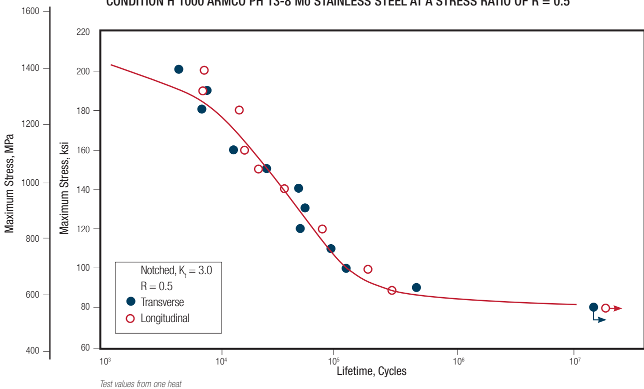
FIGURE 6 – FATIGUE TEST RESULTS FOR NOTCHED ( K_t = 3.0 ) LONGITUDINAL AND TRANSVERSE SPECIMENS OF CONDITION H 1000 ARMCO PH 13-8 Mo STAINLESS STEEL AT A STRESS RATIO OF R = 0.5
