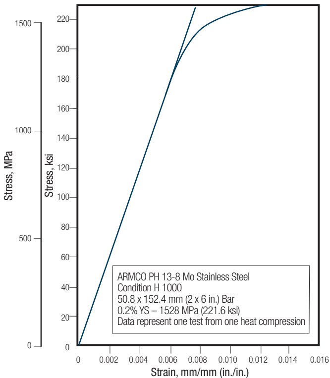
FIGURE 28 – COMPRESSION STRESS – STRAIN CURVE
