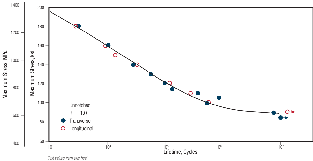
FIGURE 5 – FATIGUE TEST RESULTS FOR UNNOTCHED LONGITUDINAL AND TRANSVERSE SPECIMENS OF CONDITION H 1000 ARMCO PH 13-8 Mo STAINLESS STEEL AT A STRESS RATIO OF R = -1.0
