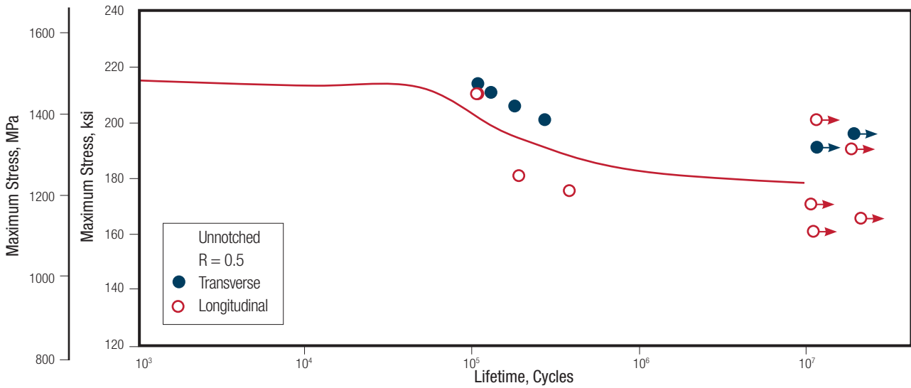
FIGURE 3 – FATIGUE TEST RESULTS FOR UNNOTCHED LONGITUDINAL AND TRANSVERSE SPECIMENS OF CONDITION H 1000 ARMCO PH 13-8 Mo STAINLESS STEEL AT A STRESS RATIO OF R = 0.5
