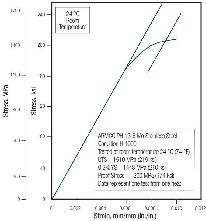
FIGURE 15 – EFFECT OF TEST TEMPERATURE ON CONDITION H 1000 – TENSION
