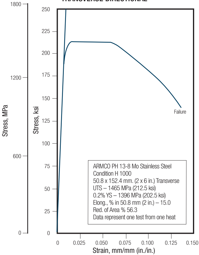
FIGURE 30 – TOTAL STRESS-STRAIN CURVES H1000 TRANSVERSE DIRECTIONAL
