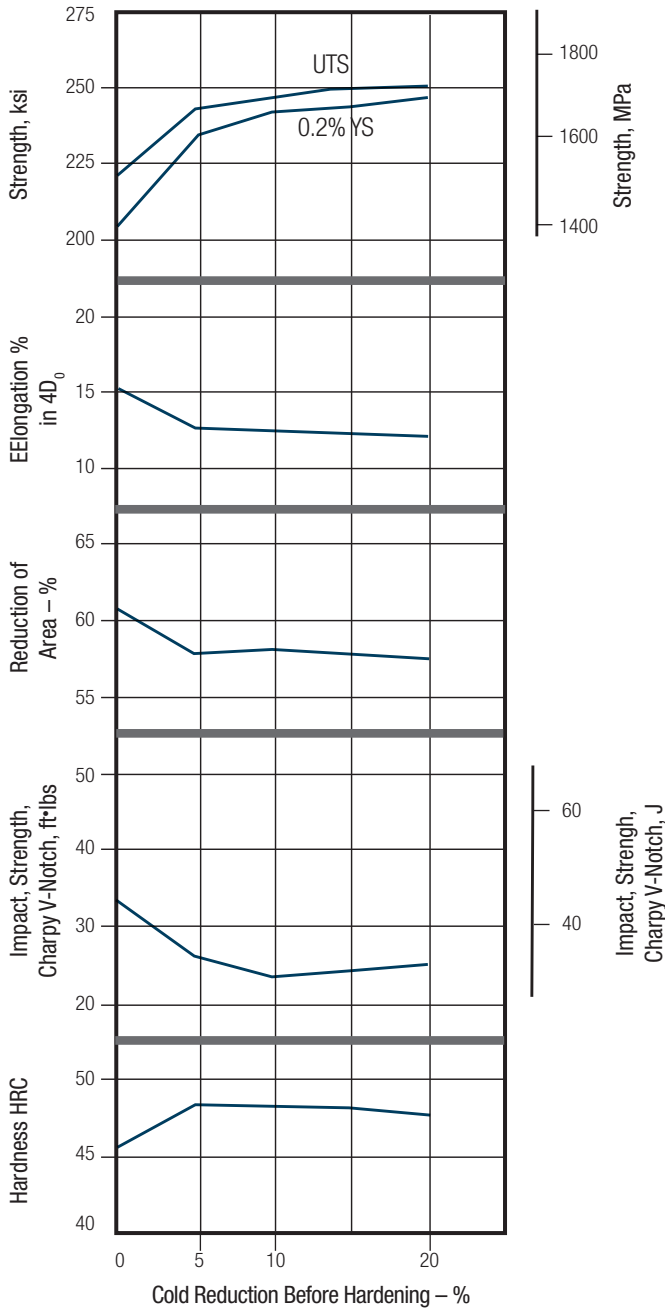
FIGURE 37 – 482 °C (900 °F) HARDENING TEMPERATURE
