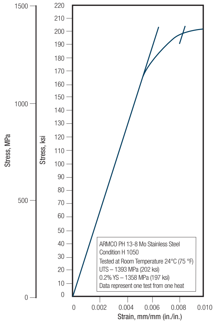
FIGURE 24 – EFFECT OF VARIOUS HEAT-TREATED CONDITIONS ON ROOM TEMPERATURE CURVES – TENSION
