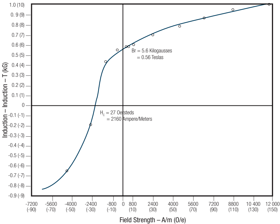
FIGURE 43 – HYSTERESIS CURVE – ARMCO PH 13-8 Mo STAINLESS STEEL – CONDITION H 950
