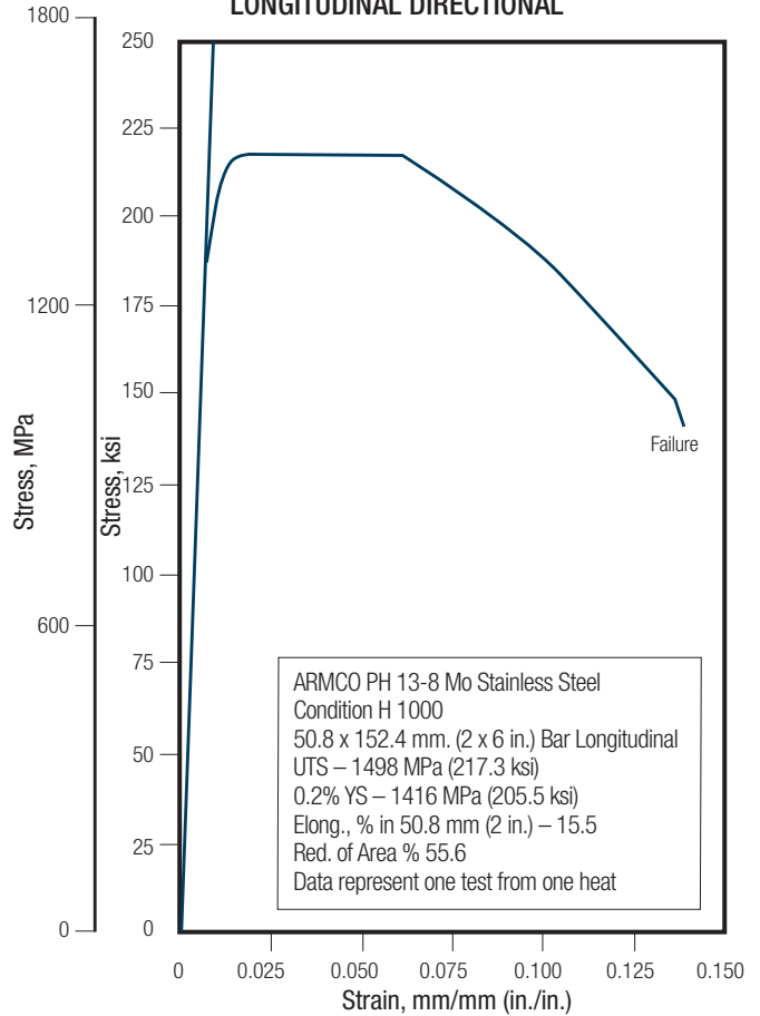
FIGURE 29 – TOTAL STRESS-STRAIN CURVES H1000 LONGITUDINAL DIRECTIONAL
