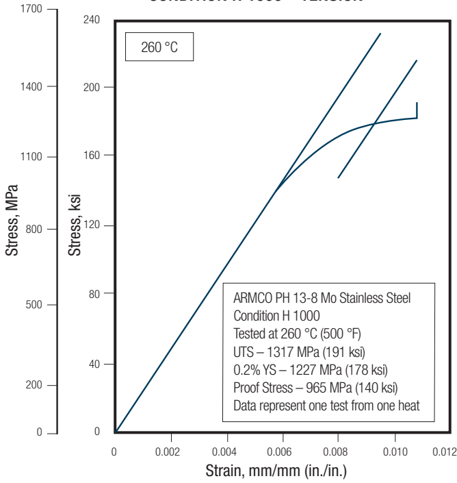
FIGURE 17 – EFFECT OF TEST TEMPERATURE ON CONDITION H 1000 – TENSION
