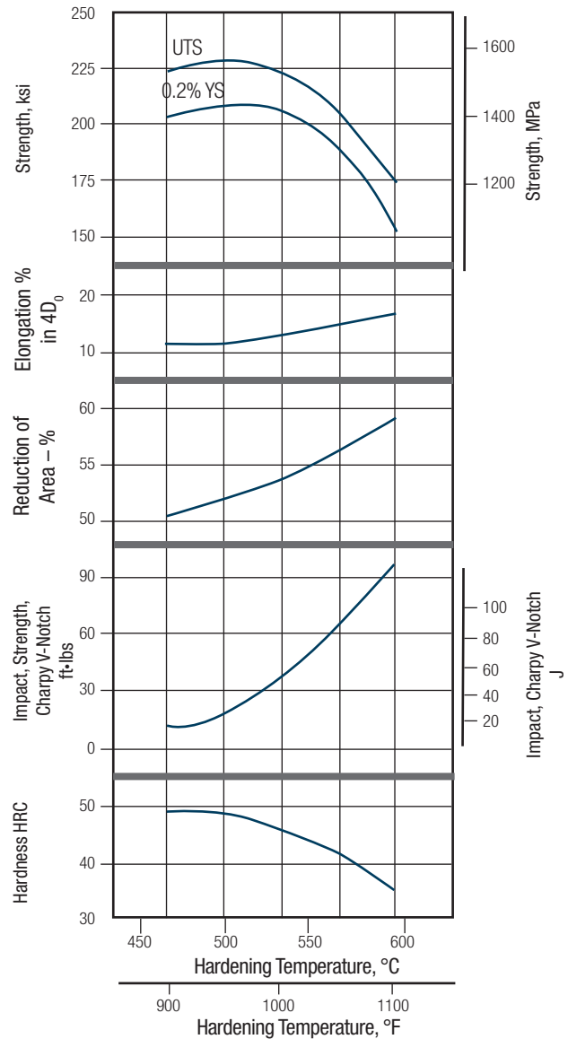
FIGURE 34 – 4 HR. HARDENING TIME, EFFECT OF VARIATION OF HARDENING TEMPERATURE*
