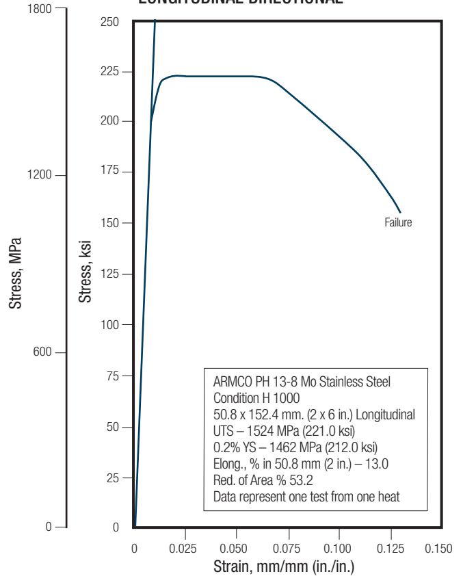
FIGURE 31 – TOTAL STRESS-STRAIN CURVES H1000 LONGITUDINAL DIRECTIONAL
