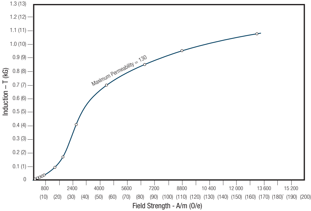
FIGURE 42 – NORMAL INDUCTION – ARMCO PH 13-8 Mo STAINLESS STEEL – CONDITION H 950
